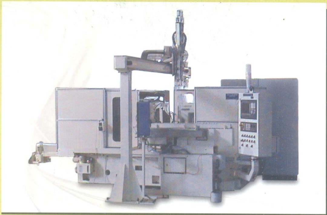
Bocca 7 Axis CNC "UJ Cross" Centerless Grinder – 2 parts simultaneously with Gantry Loader.
